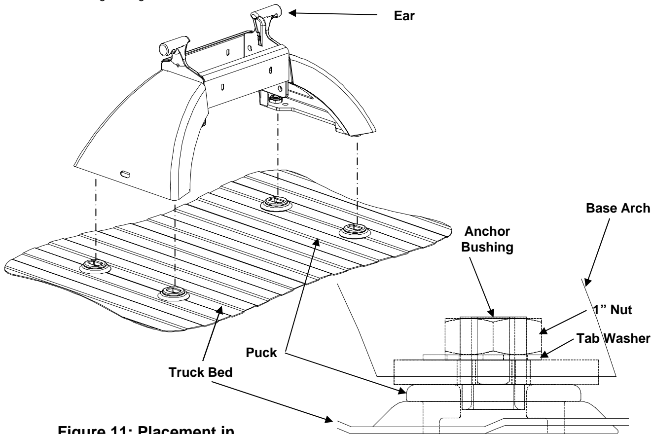
Figure 11: Placement in Mounting Kit / Truck Bed
