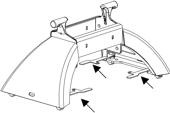
Figure 14A: Anchor Handles in Unlocked Position
