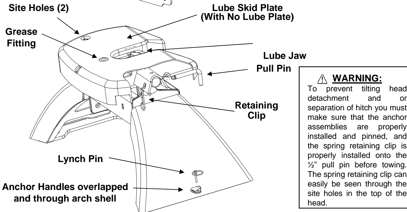
Figure 21 : Pin and Clip (Skid Plate cut away view)
