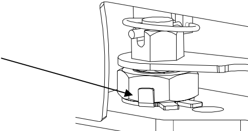
Figure 16: Bending Up Tab to Flat of Nut
