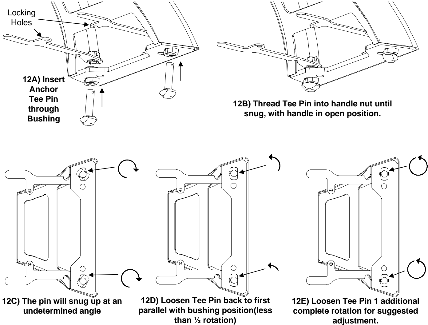
Figure 12 : Anchor Tee Pin and Handle Orientation(all shown in unlocked position)
